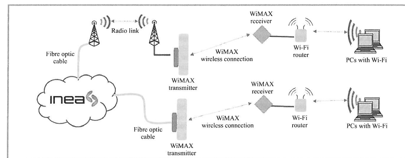
Fig. 3. General topology of INEA WiMAX network.
